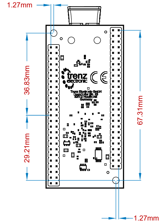
View from Bottom side (Scale 1:1)
