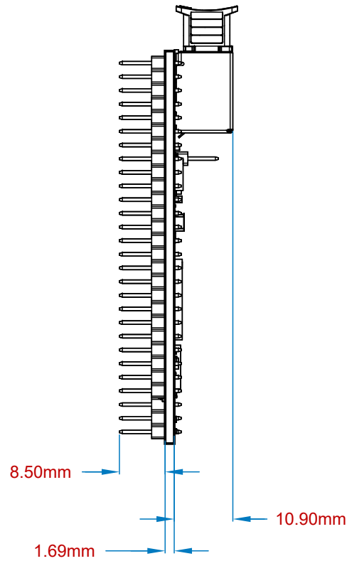
View from Left side (Scale 1:1)
