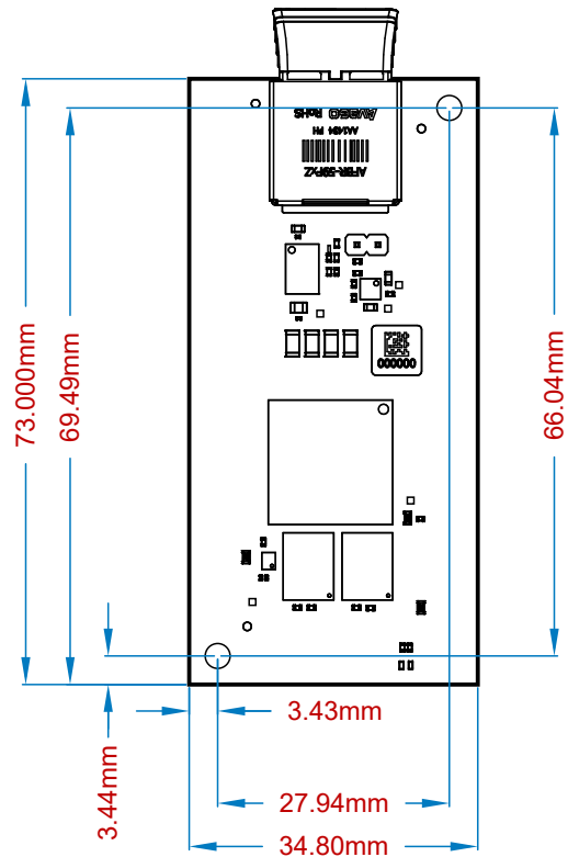
View from Top side (Scale 1:1)
